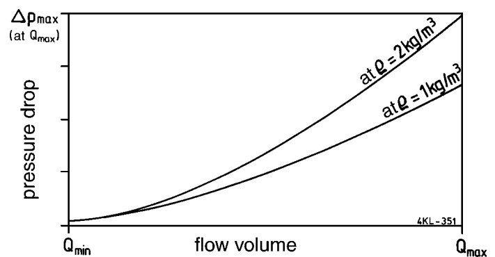
Typical pressure drop diagram for gas specific weights \rho = 1 \text{ kg/m}^3 and \rho = 2 \text{ kg/m}^3 .
